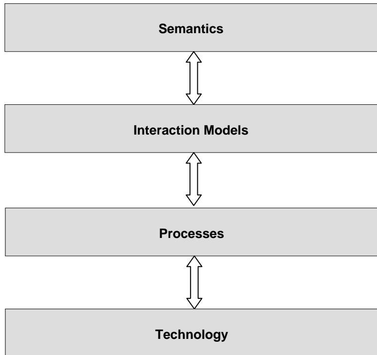
Figure 1: eInvoicing Framework
